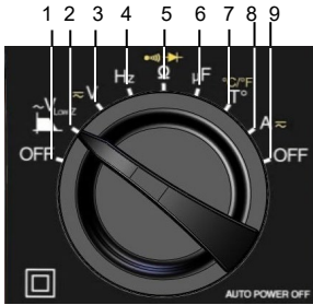
Figure 1: the switch
